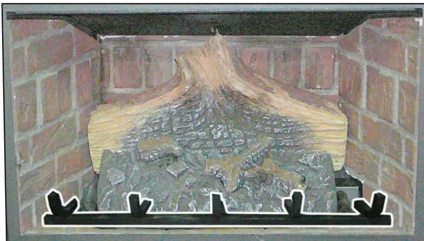
Figure 46: Third Stage Log Set Installation.
