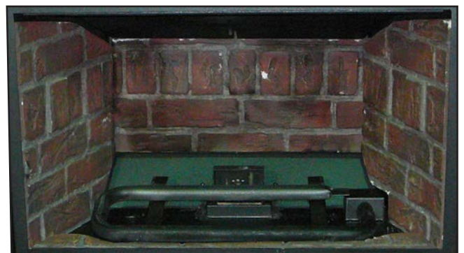
Figure 43: The firebox showing the brick panels and burner tube already installed.
