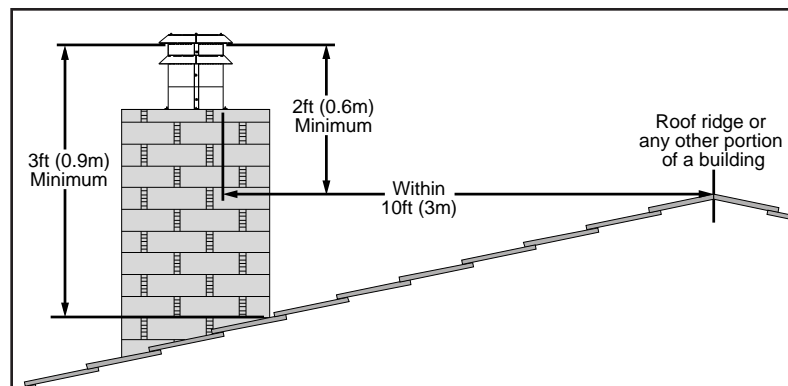
Figure 17: Roof Clearances.
