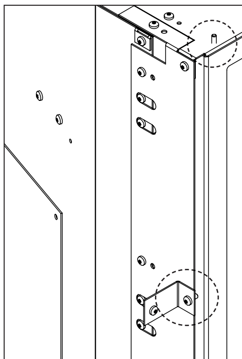
Figure 33: Panel Bracket Installed and Pin Location
