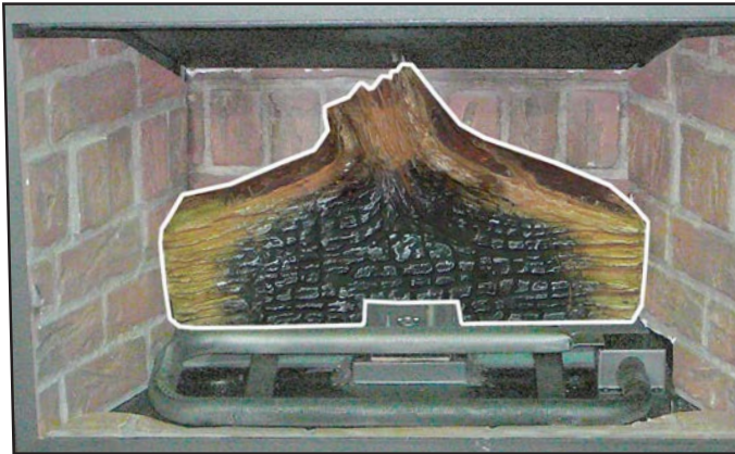
Figure 44: First Stage Log Set Installation.
