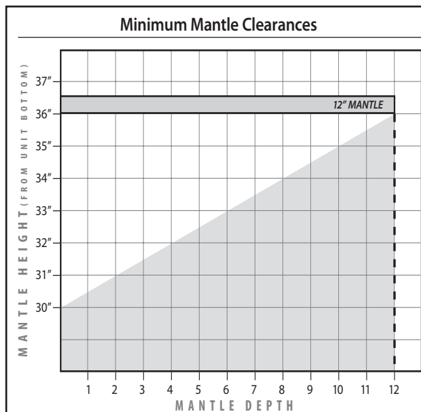
Figure 16: Mantle width and height.
