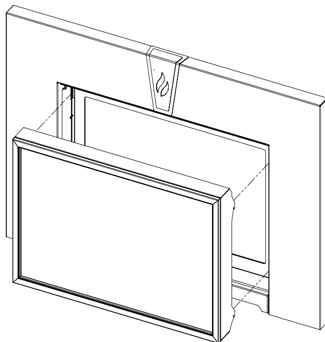
Figure 37: Installing Safety Screen onto Brackets.
