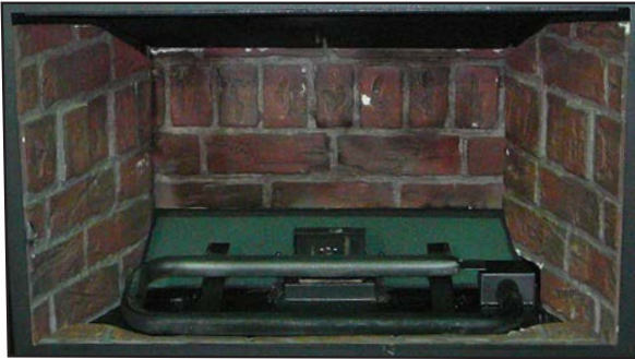
Figure 38: Carefully remove the front brick panel on the bottom of the firebox by lifting it up.
