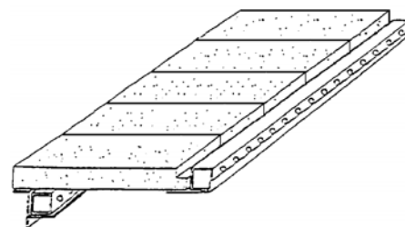
Side View of Baffle Brick Installed
