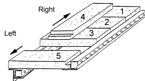
Top View of Baffle Brick Installed
